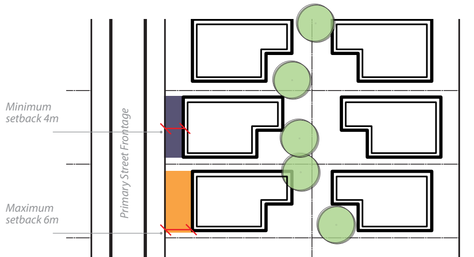
STANDARD LOT SETBACK PLAN
